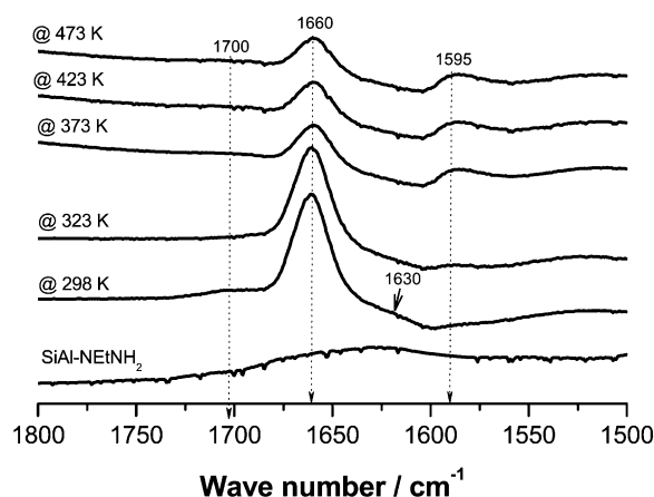
Figure 3. In situ FTIR spectra of the Si–Al– \text{NHCH}_2\text{CH}_2\text{NH}_2 catalyst using butan-2-one as a probe molecule at different reaction temperatures.
